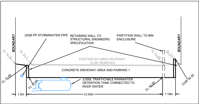
S4 - EXTERNAL PARKING SECTION
