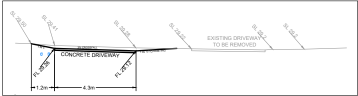
S2 - DRIVEWAY ACCESS SECTION
