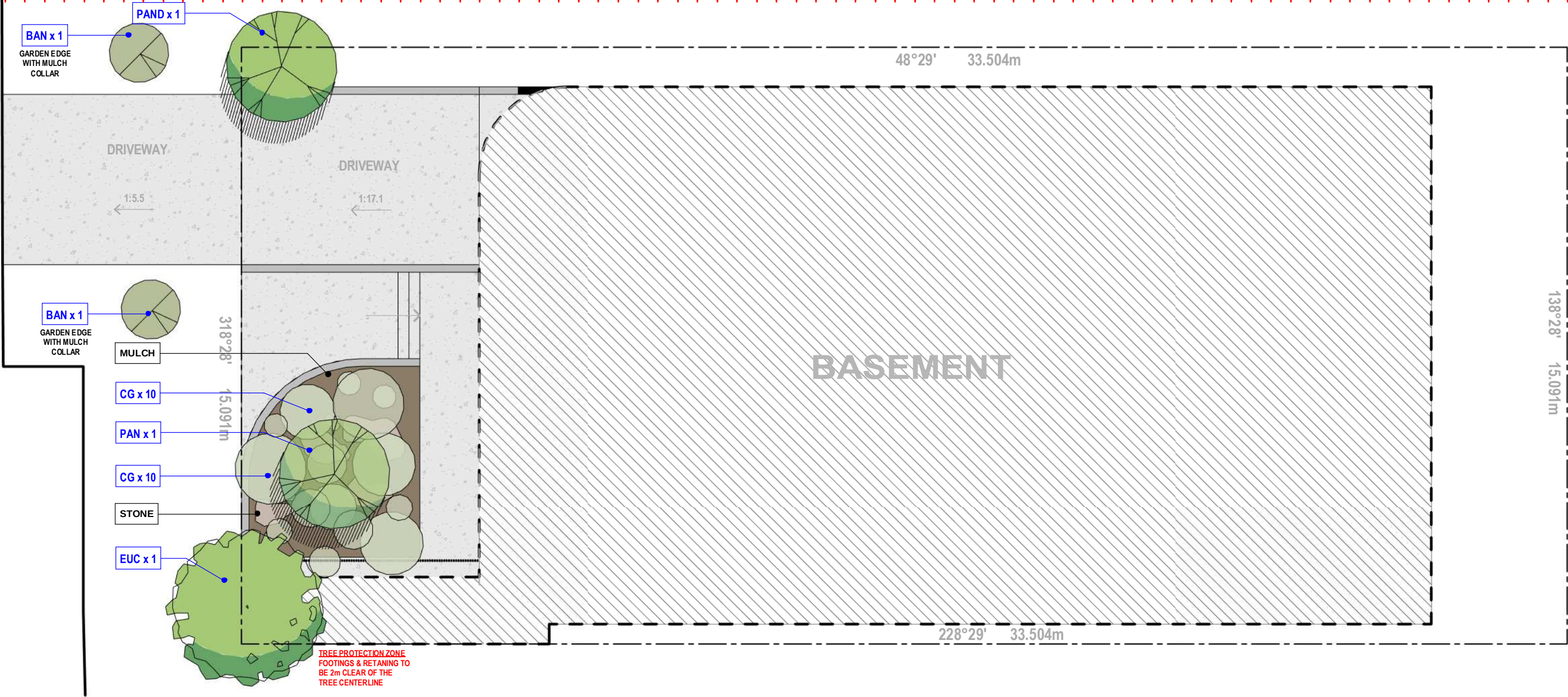
Plan BASEMENT LANDSCAPE PLAN 1 : 100
