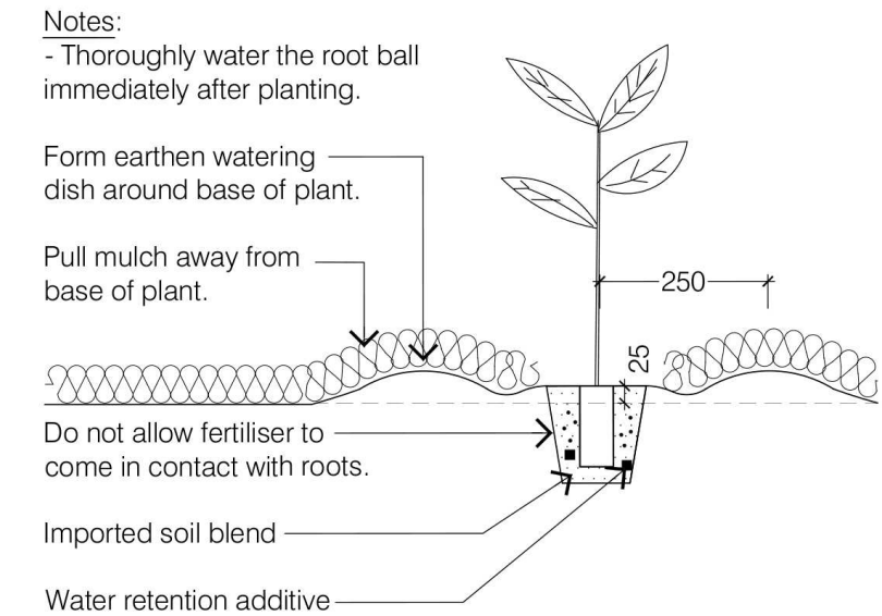
1 PLANTING DETAIL: TUBESTOCK
