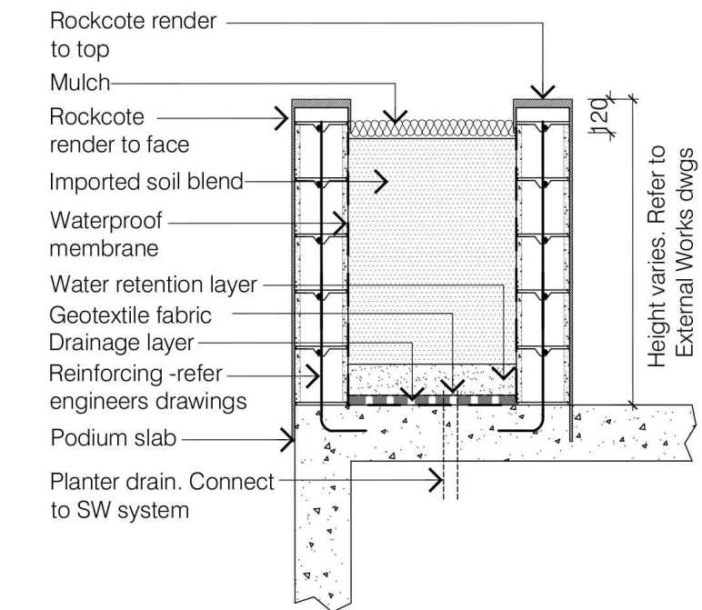
4 PODIUM PLANTING DETAIL
