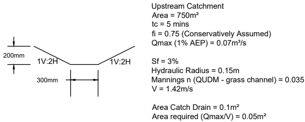
DETAIL D - TURFED CATCH DRAIN SCALE: NTS
