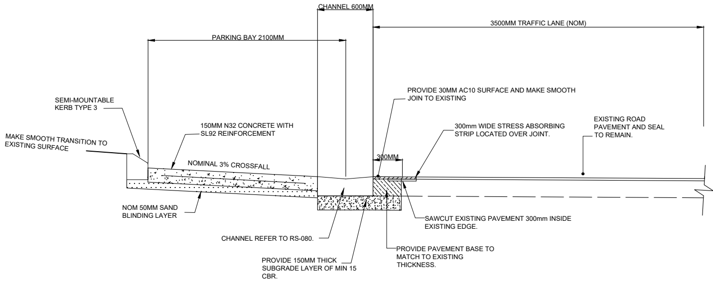
DETAIL E - ON STREET PARKING SECTION SCALE: NTS
