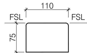
5 EDGE TYPE 1 - EXTRUDED CONCRETE
