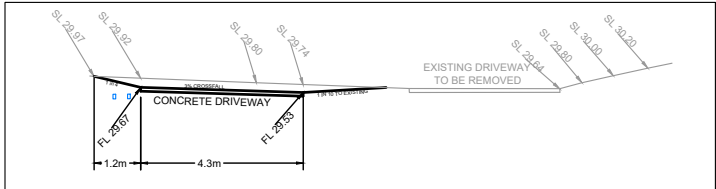
S3 - DRIVEWAY ACCESS SECTION
