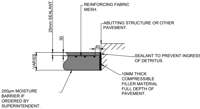
DETAIL B- ISOLATION JOINT (IJ) SCALE: 1:16
