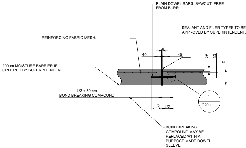
DETAIL C - EXPANSION JOINT (EJ) SCALE: 1:16
