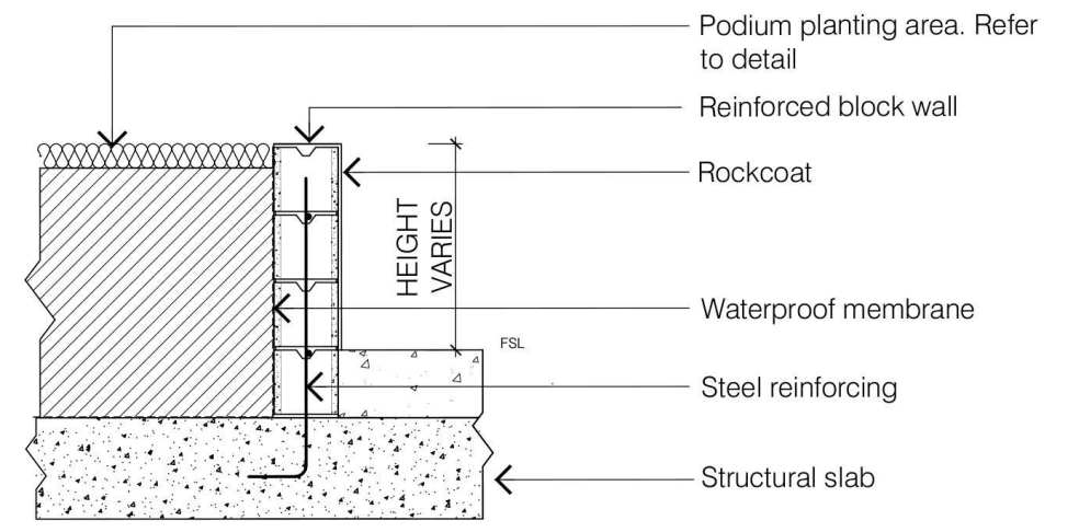
8 WALL TYPE 1
