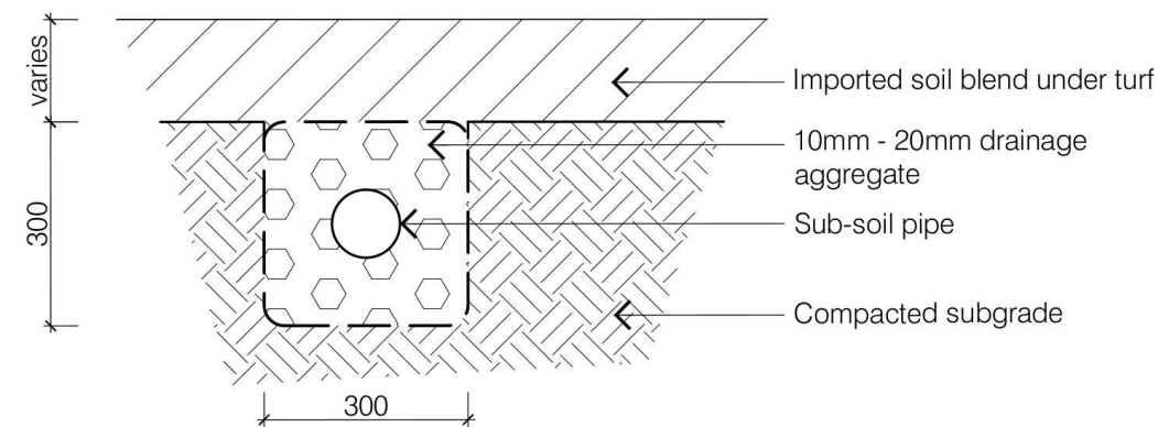
7 SUB SOIL DRAINAGE
