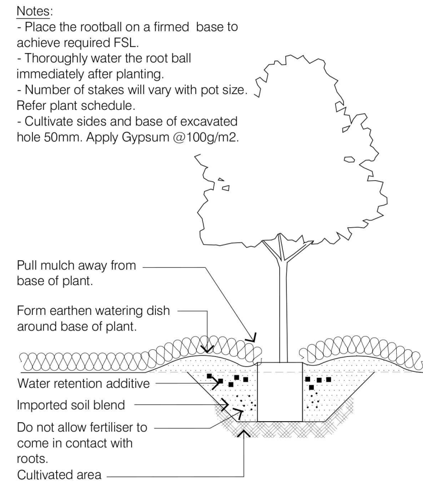
2 PLANTING DETAIL: 140-300mm
