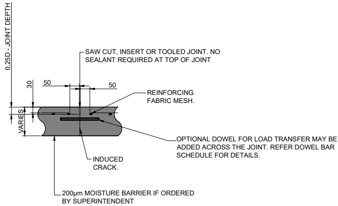
DETAIL A - CONTROL JOINT (CJ) SCALE: 1:16
