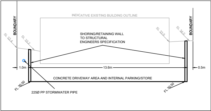
S5 - INTERNAL PARKING SECTION
